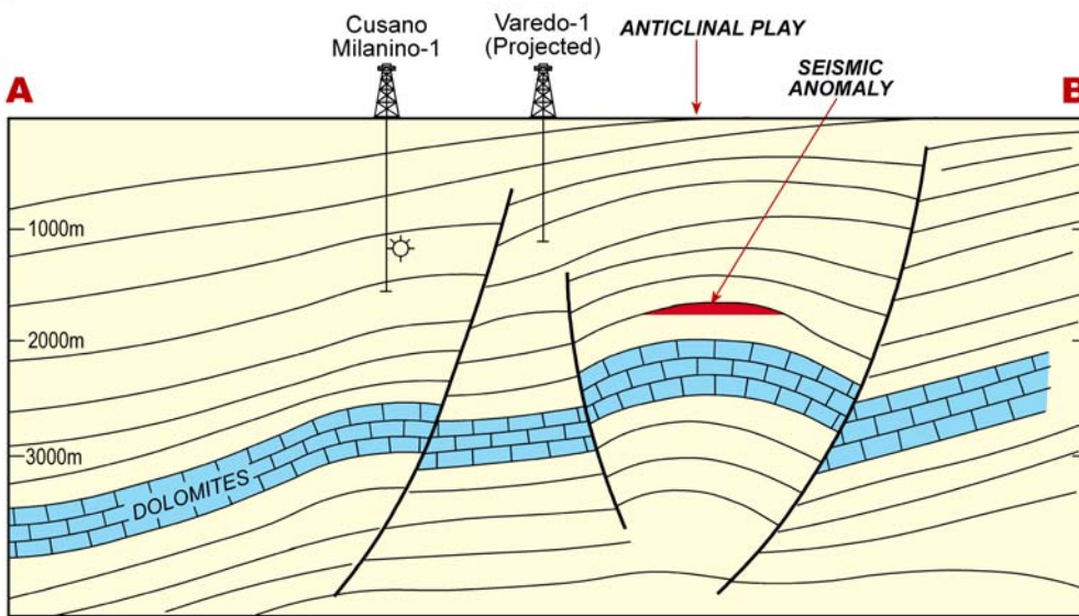
Schematic Cross Section
